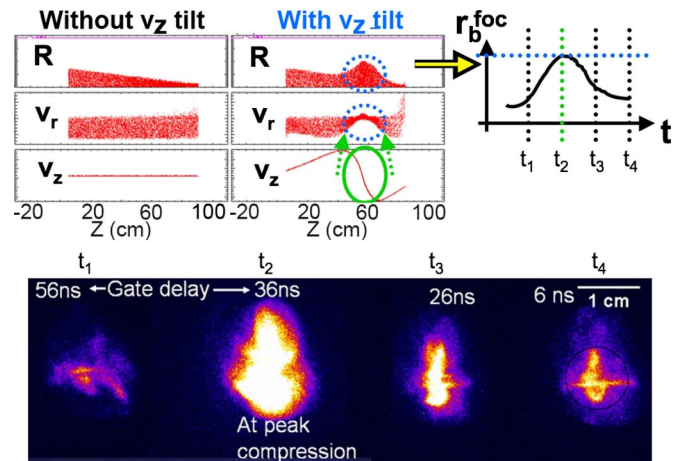
FIG. 12. (Color online) Beam phase space comparison (top) between transverse focusing without (left) and with (middle) a v_z(t) tilt. Excess divergence is imparted to the beam (right), such that the time of best longitudinal focus coincides with the worst transverse focus. Scintillator images corroborated this effect in NDCX experiments (bottom).
