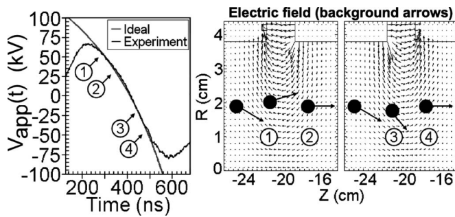
FIG. 11. Illustration of the transverse defocusing effect of the gap during the dV_{\text{app}}(t)/dt < 0 portion of the voltage waveform for longitudinal compression.
