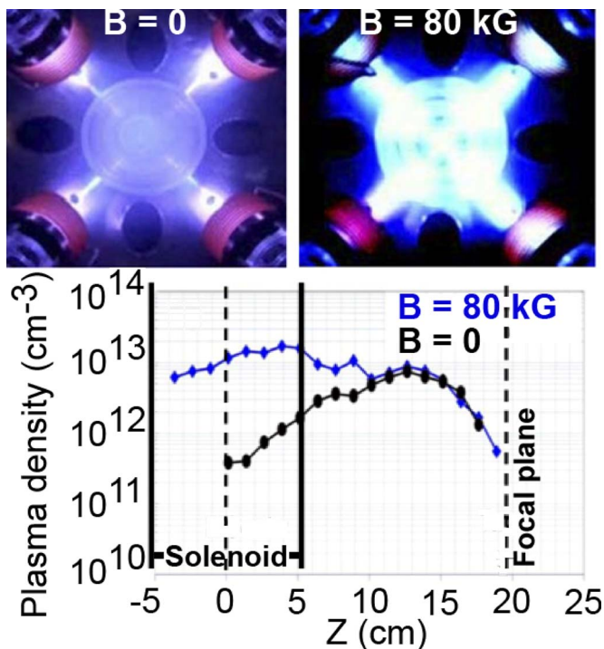
FIG. 18. (Color online) Digital camera pictures of an arrangement of four FCAPSs in operation without (top left) and with (top right) a powered final-focus solenoid. The magnetic fringe fields of the solenoid act as guide channels for the plasma flow, and the strong field compresses the plasma density.
