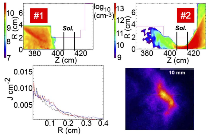
FIG. 17. (Color online) Plasma density ( \log_{10} scale) of main drift length plasma (top left) and FCAPS injection (top right) into a final-focus solenoid (marked “Sol.”) with length \sim 10 cm and strength B_z \sim 50 kG. The simulation predicts a spot size of r_b^{\text{foc}} \sim 2 mm (bottom left) and agrees well with the transverse scintillator image of the simultaneously focused beam at time of peak longitudinal compression (bottom right).
